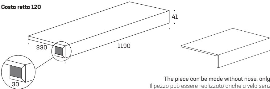
Costa retta 120
