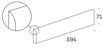
Battiscopa 60 #12mm
