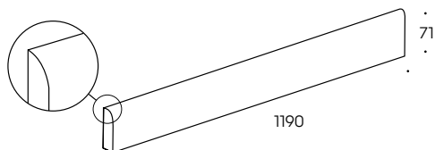
Battiscopa 120 ≈6mm
